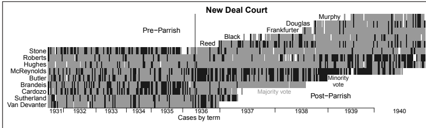
Figure 1. Votes in all nonunanimous cases for the 1931–1940 terms. Justices on the y-axis are sorted by years of service and cases are sorted by dates of decision. Grey (black) cells indicate a majority (minority) vote. The vertical line denotes the Parrish case, decided in the 1936 term, with a formal decision issued on March 29, 1937. This figure demonstrates a marked rupture in voting patterns around the time of the case.
