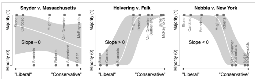
Figure 3. Modeling the probability of judicial votes as a function of a latent dimension. The x-axis represents the latent dimension. The y-axis represents the probability of a vote for the majority, ranging from 0 to 1. The grey dots are the observed votes by each justice. The white lines represent the estimated probability as a function of the latent dimension (with 95% credibility bands). A positive slope means that the majority is estimated to be "conservative" and a negative slope means that the majority is estimated to be "liberal." The steepness of the slope reflects how much we learn about differences in the ideal points of the justices. Since slopes are not equal, cases contribute differentially to ideal points. Snyder v. Massachusetts in the left panel features an atypical majority coalition and thus has a slope that is not statistically different from 0. It therefore contributes little information about the ideal points. Helvering v. Falk on the other hand, has a sharp positive slope reflecting the larger amount of information this case contains for our estimation strategy. Nebbia v. New York contributes a similar amount of information, although here there is a liberal majority and hence a negative slope.
