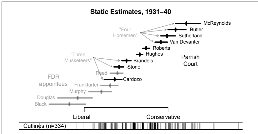
Figure 5. Static (median) ideal point estimates with 95% credible intervals for the 1931-40 terms. Justices are sorted from left to right by median ideal point. Ideal points for justices serving on or before the Parrish term are plotted in black, and others in grey. Bottom strip presents estimated splits between the majority in minority in 334 cases ( \kappa : from Appendix A). Static ideal points capture key conventional understandings of the jurisprudence of these justices—i.e., the major cleavages in the Parrish Court between the “Four Horsemen” and the “Three Musketeers”; the center of the Court occupied by Roberts and Hughes; and the liberal turn of the Roosevelt appointees.
