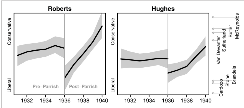
Figure 13. This figure plots dynamic ideal points with separate pre and post-Parrish trends for Justice Roberts and Chief Justice Hughes. The solid lines represent the pointwise posterior median ideal points and the grey bands provide pointwise 95% credible regions. Justice Roberts and, to a lesser extent, Chief Justice Hughes experience sharp shifts to the left in the 1936 term. For reference, arrows on the right provide posterior median ideal points of justices other than Roberts and Hughes on the Court in the 1936 term.
